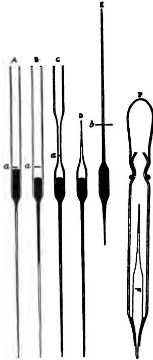
FIG. 19.—Making throttle pipettes—large capacity
